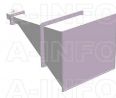
LB-340-20-C-7/16FSPO Standard Gain Horn Antenna 2.2-3.3GHz 20dB Gain 7/16(DIN) Female
